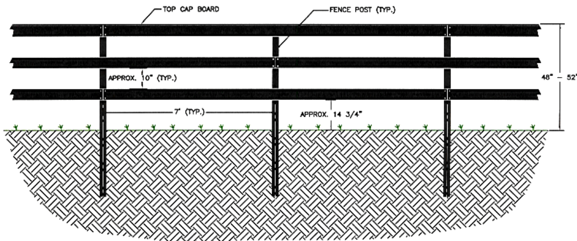
FENCING DETAIL
