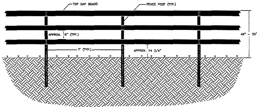
FENCING DETAIL
